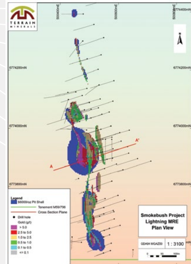
Diagram 2: Plan View of Lightning Inferred Mineral Resource Estimation with $6,000/oz optimised pit shell.
