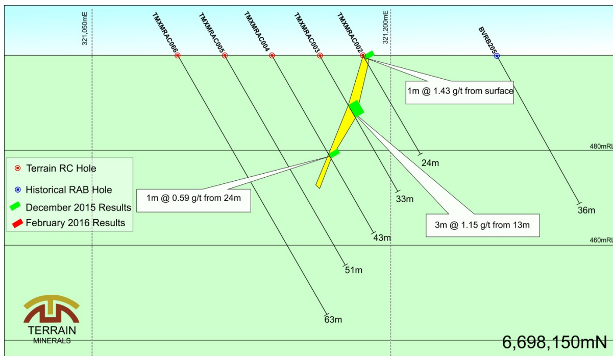
Figure 4: Drill Section 6,698,150mN
