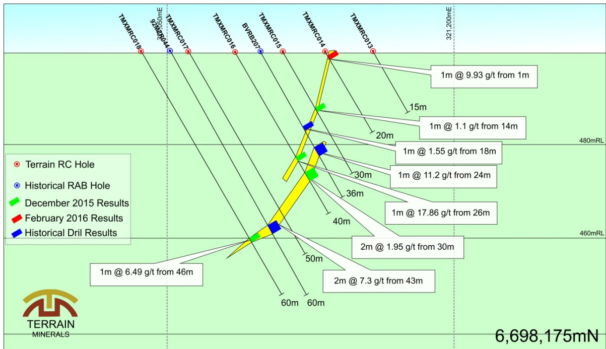
Figure 1: Drill Section 6,698,175mN
