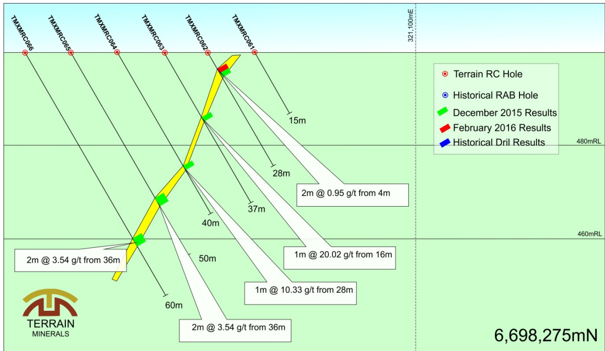
Figure 9: Drill Section 6,698275mN
