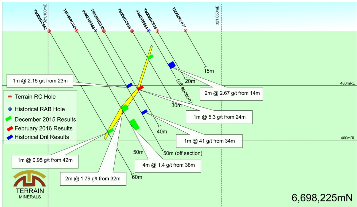
Figure 7: Drill Section 6,698,225mN
