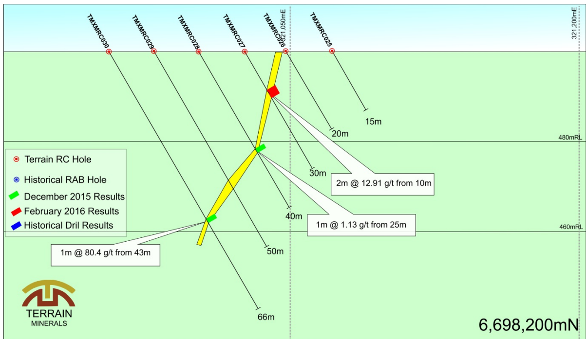
Figure 6: Drill Section 6,698,200mN
