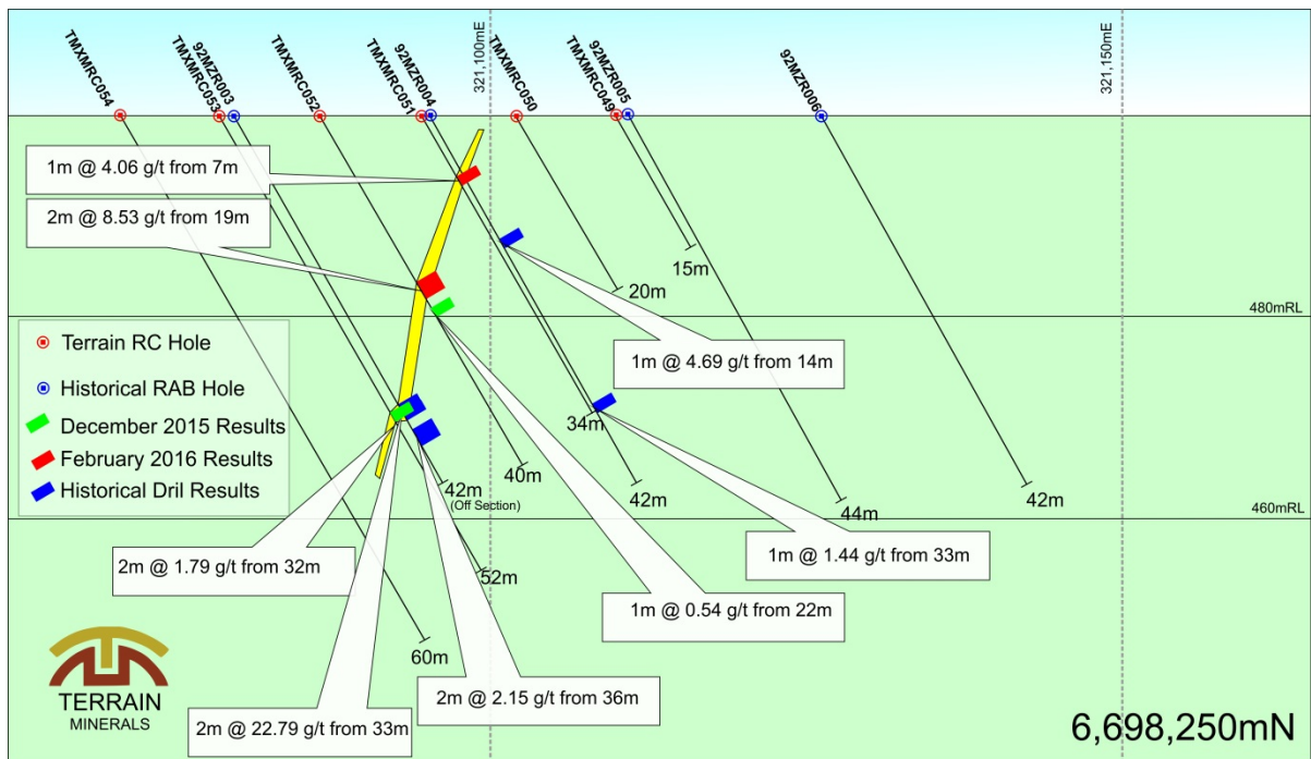
Figure 8: Drill Section 6,698,250mN
