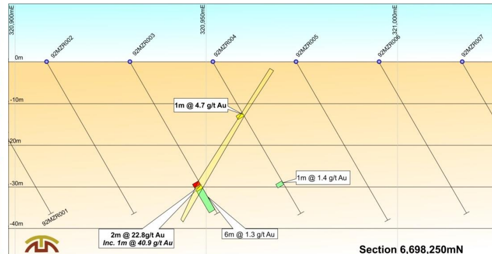
Section 6,698,250mN
